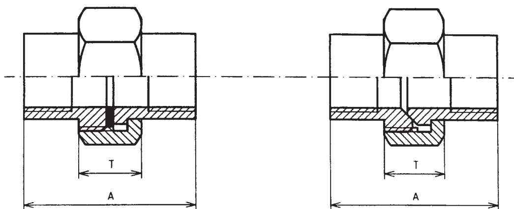
Socket union with flat seat
