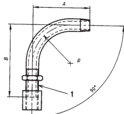
1 Parallel thread length as for long screw Type 1A
