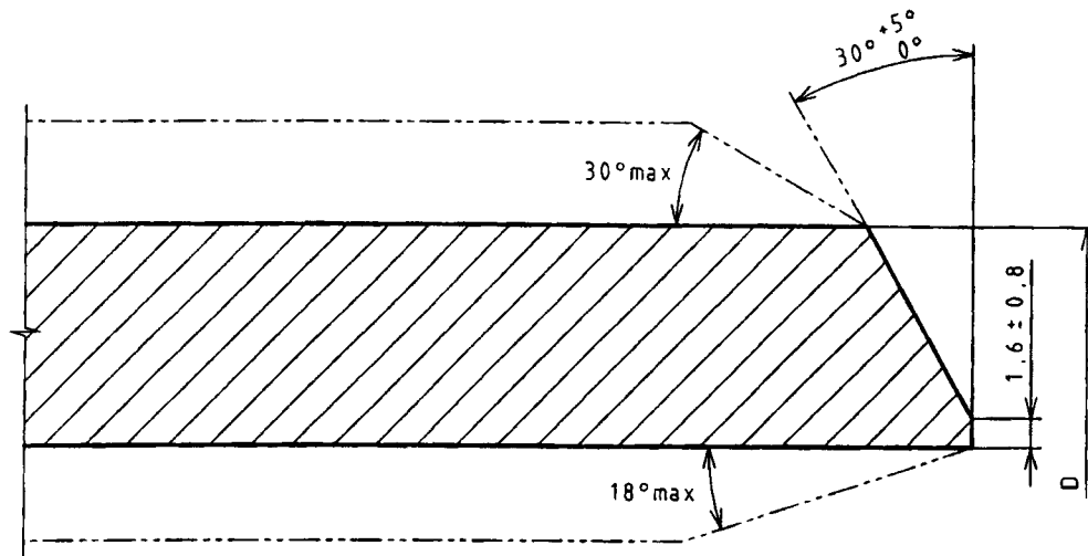
Figure 12 — End finishing
