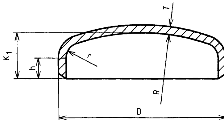
Figure 9 — Dished end
