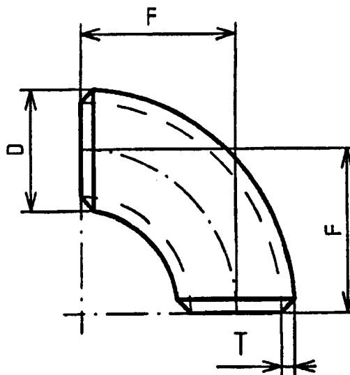
Figure 2 — 90° Elbow
