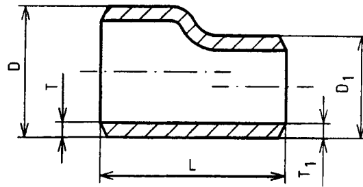
Figure 6 — Eccentric reducer
