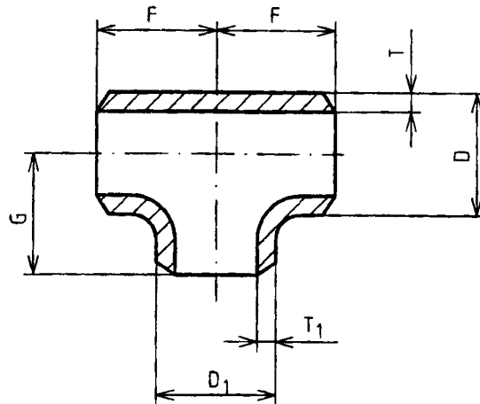
Figure 8 — Reducing tee
