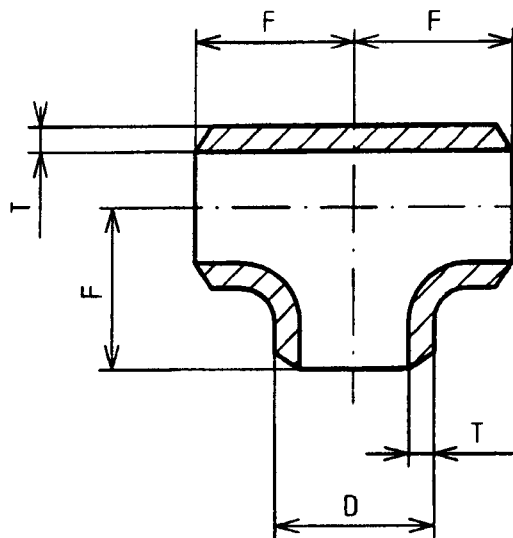
Figure 7 — Equal tee
